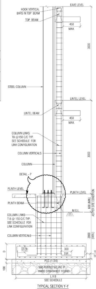
TYPICAL SECTION Y-Y NOT TO SCALE
