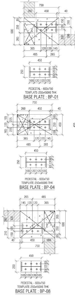
ANCHOR BOLT DETAILS ALL COLUMN BOLTS QTY. NO. OF BOLT 120 NOS.
