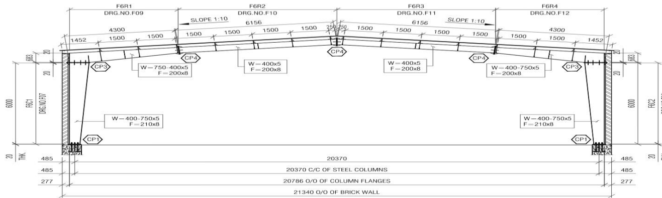
FRAME-6 (1 NO. REQUIRED) SCALE 1:125
