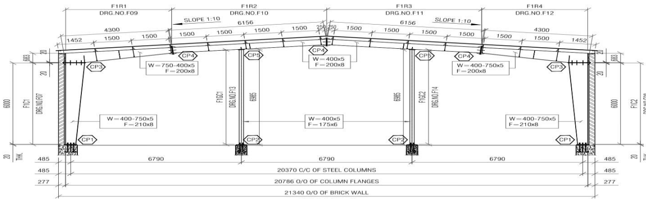
FRAME-1 (1 NO. REQUIRED) SCALE 1:125
