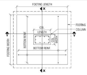
TYPICAL FOOTING PLAN DETAILS NOT TO SCALE
