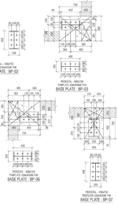
ANCHOR BOLT DETAILS ALL COLUMN BOLTS QTY. NO. OF BOLT 120 NOS.
