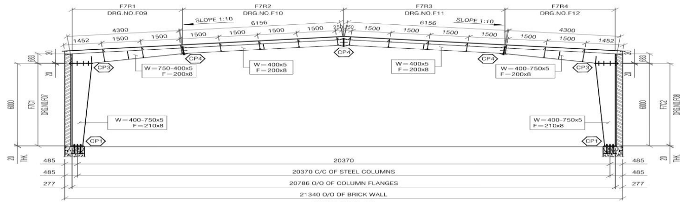
FRAME-7 (1 NO. REQUIRED) SCALE 1:125
