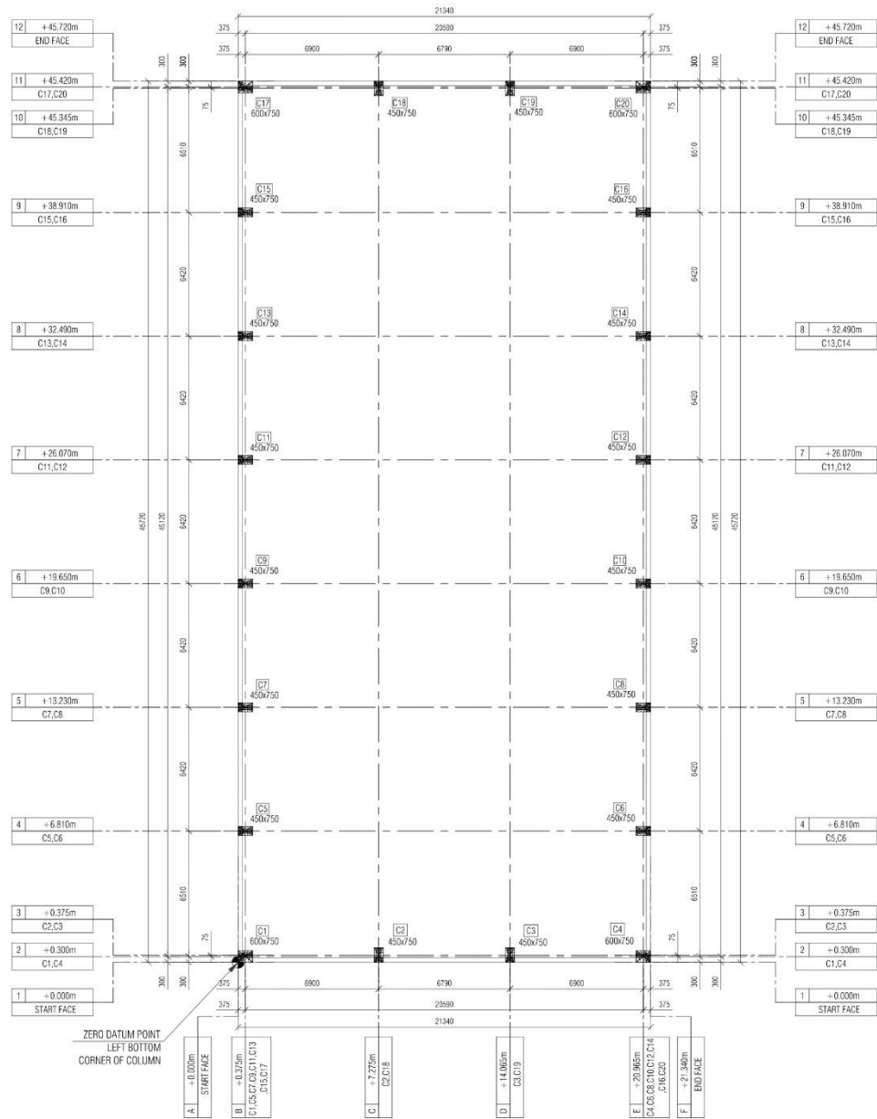
RC COLUMN CENTER LINE DETAILS SCALE 1:150
