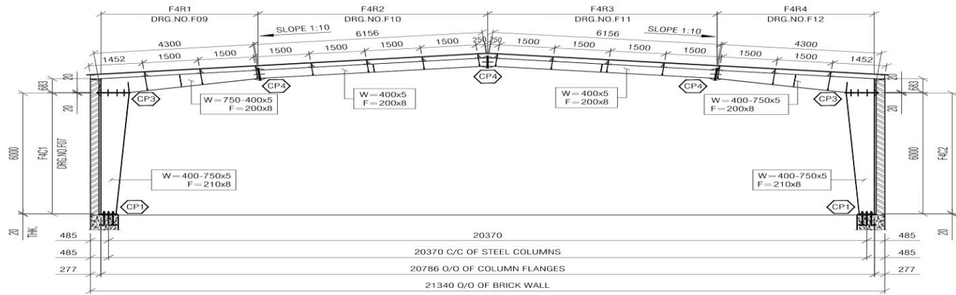
FRAME-4 (1 NO. REQUIRED) SCALE 1:125
