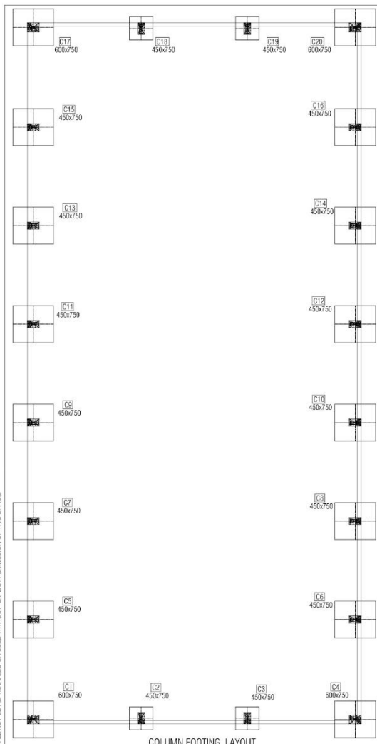
COLUMN FOOTING LAYOUT SCALE 1:150
