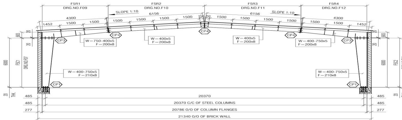
FRAME-5 (1 NO. REQUIRED) SCALE 1:125
