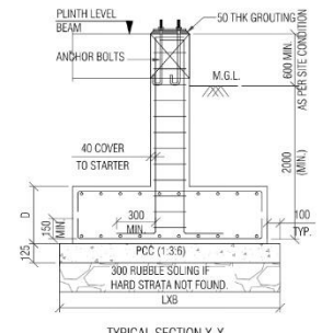
TYPICAL SECTION X-X NOT TO SCALE
