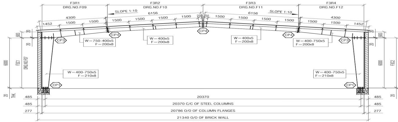
FRAME-3 (1 NO. REQUIRED) SCALE 1:125
