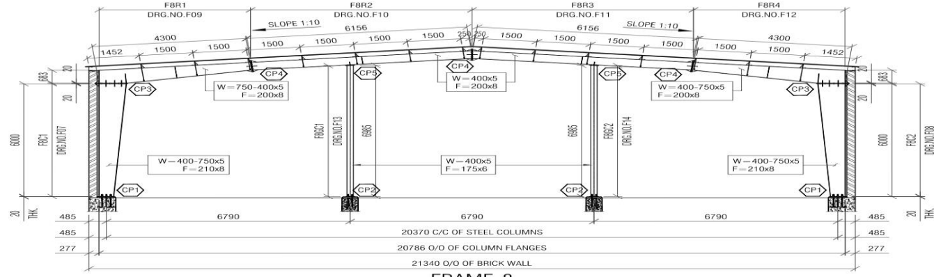
FRAME-8 (1 NO. REQUIRED) SCALE 1:125
