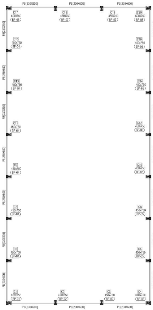
PLINTH BEAM LAYOUT SCALE 1:150
